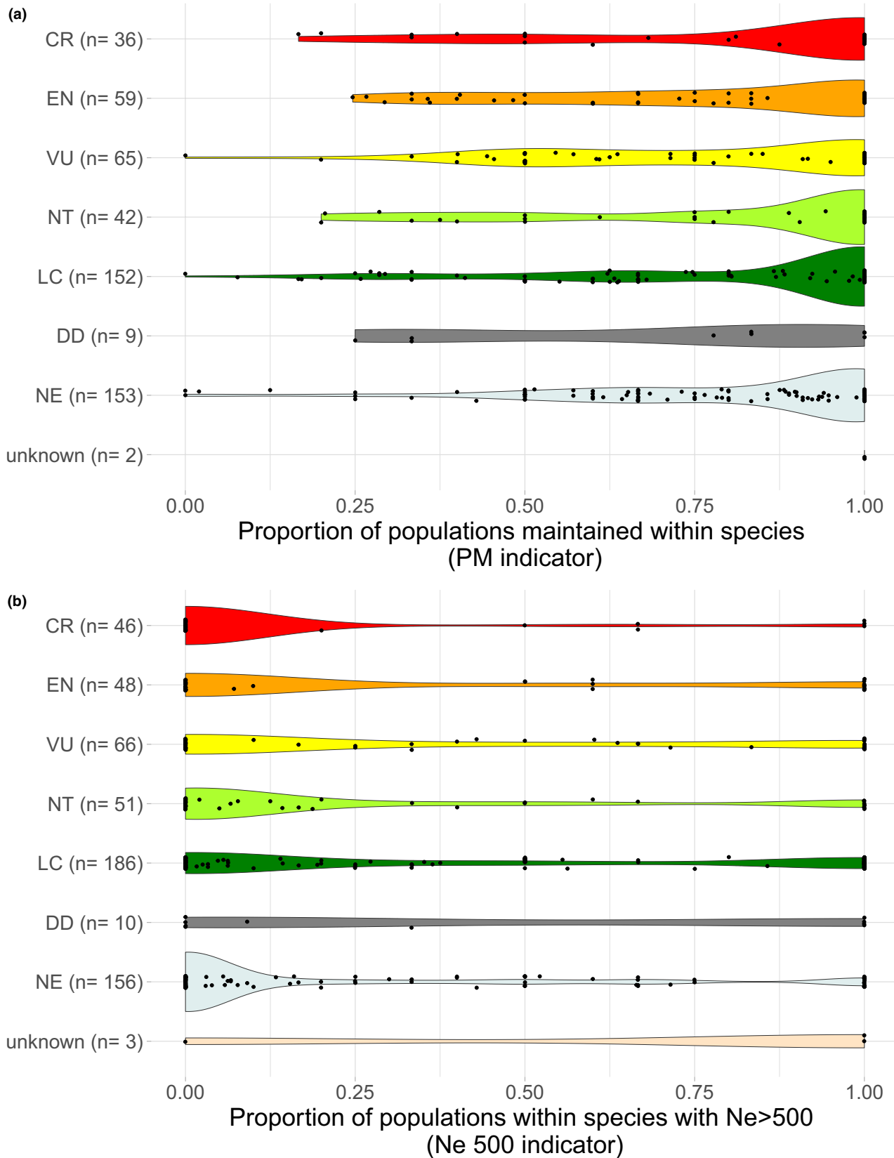
FIGURE 5 Violin plots illustrating the spread in (a) PM and (b) N_e > 500 indicator values across IUCN Red List categories. Species were classified by their Global Red List status. Abbreviations reflect official IUCN Red List categories. Sample sizes ( n ) are provided for each threat category.
